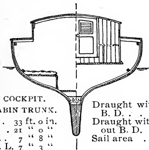
SEAWANHAKA KNOCKABOUT.
